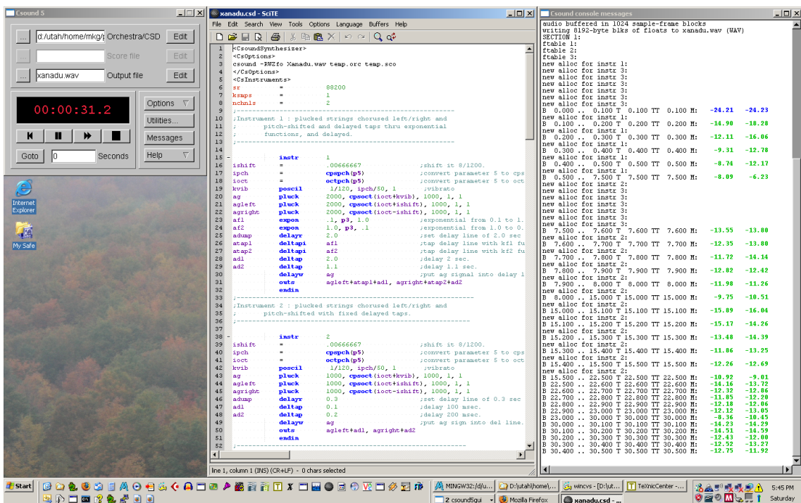
Figure 2.14.: GUI Rendering
