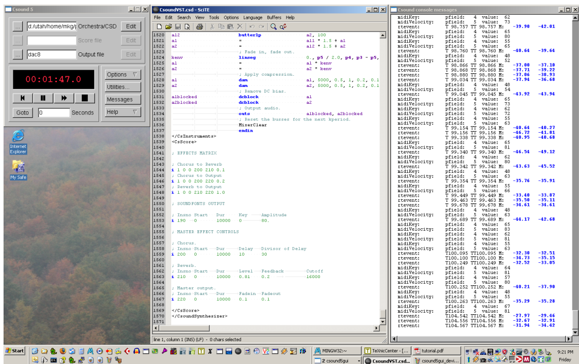
Figure 2.17.: MIDI Performance
