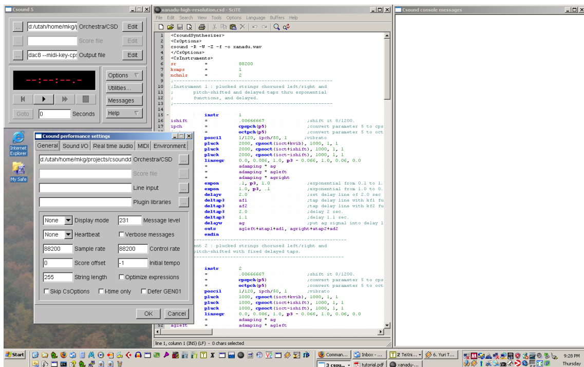
Figure 2.13.: General Options
