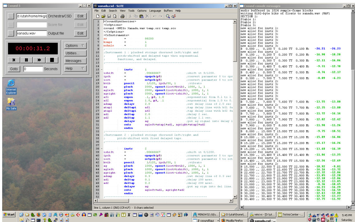
Figure 2.14.: GUI Rendering
