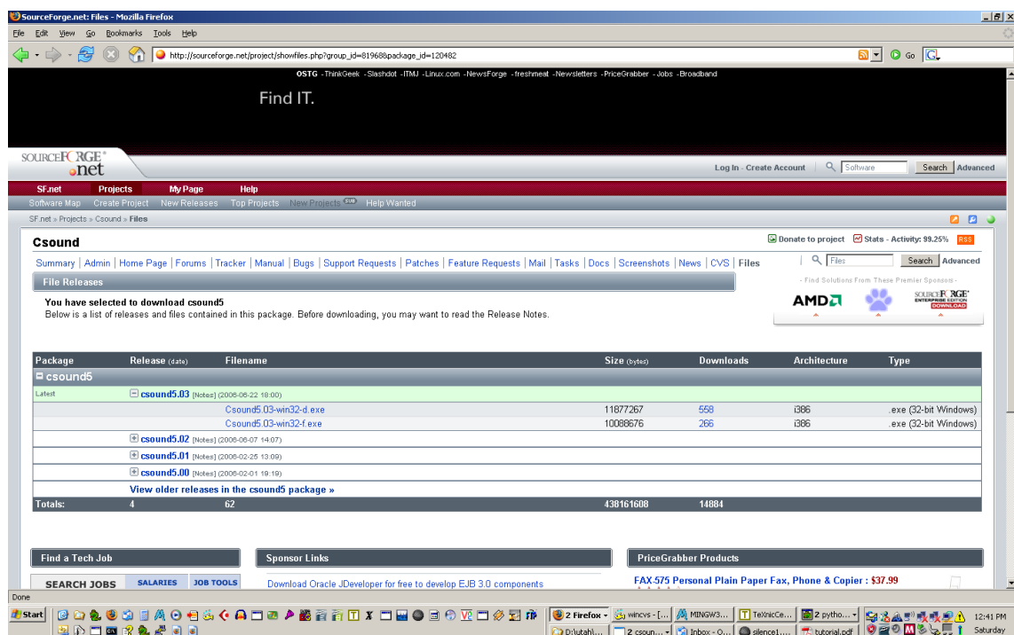
Figure 2.1.: Download Page
