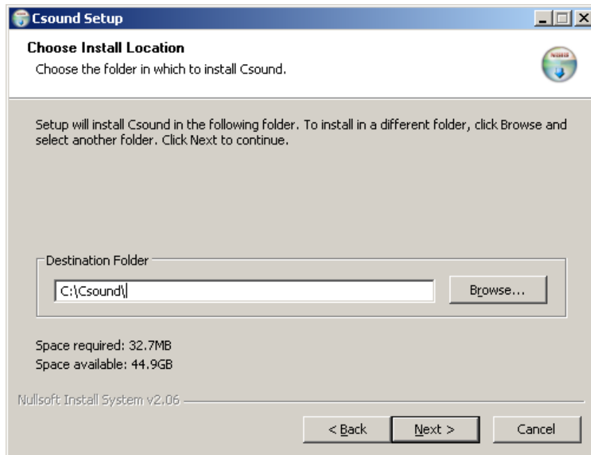
Figure 2.4.: Csound Location
