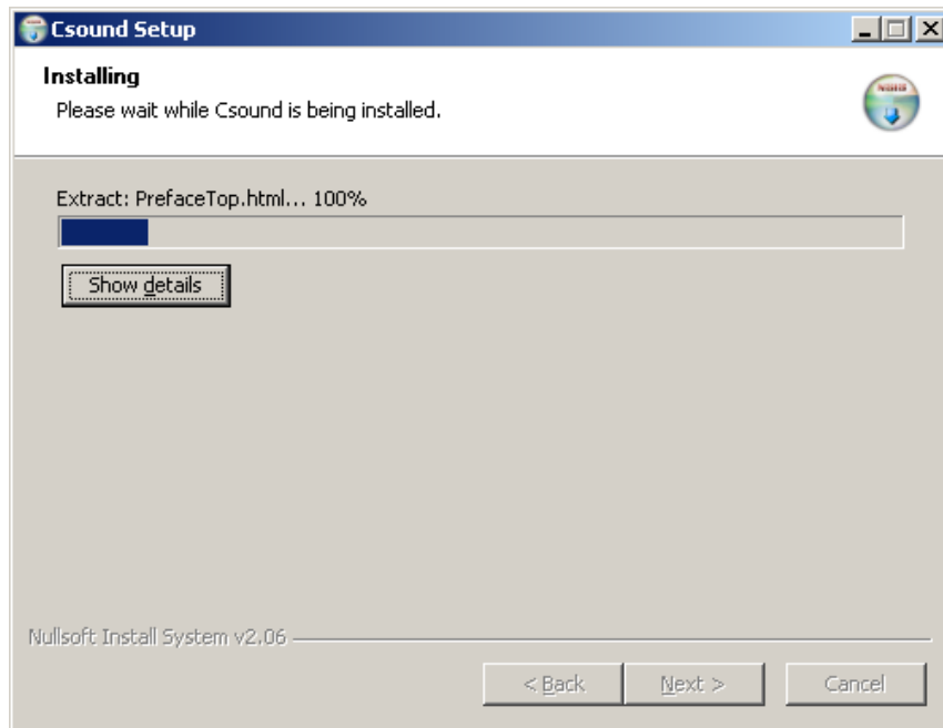
Figure 2.6.: Csound Installing
