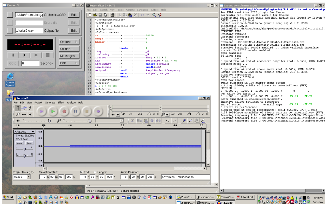
Figure 3.1.: tutorial2.csd
