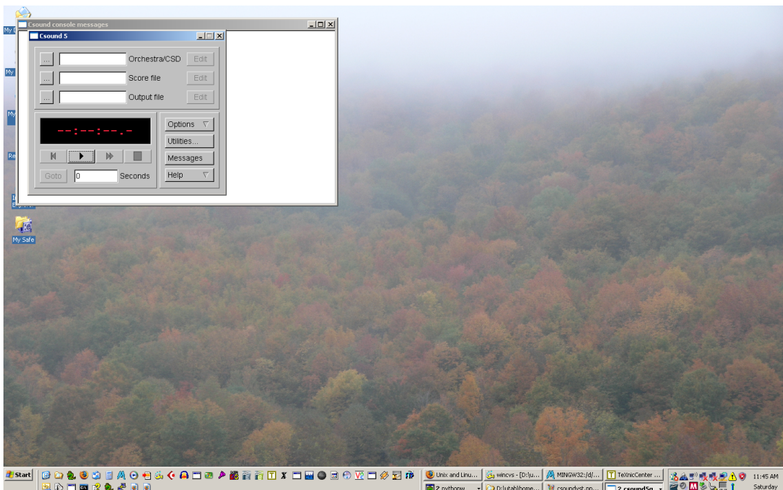
Figure 2.9.: Csound GUI
