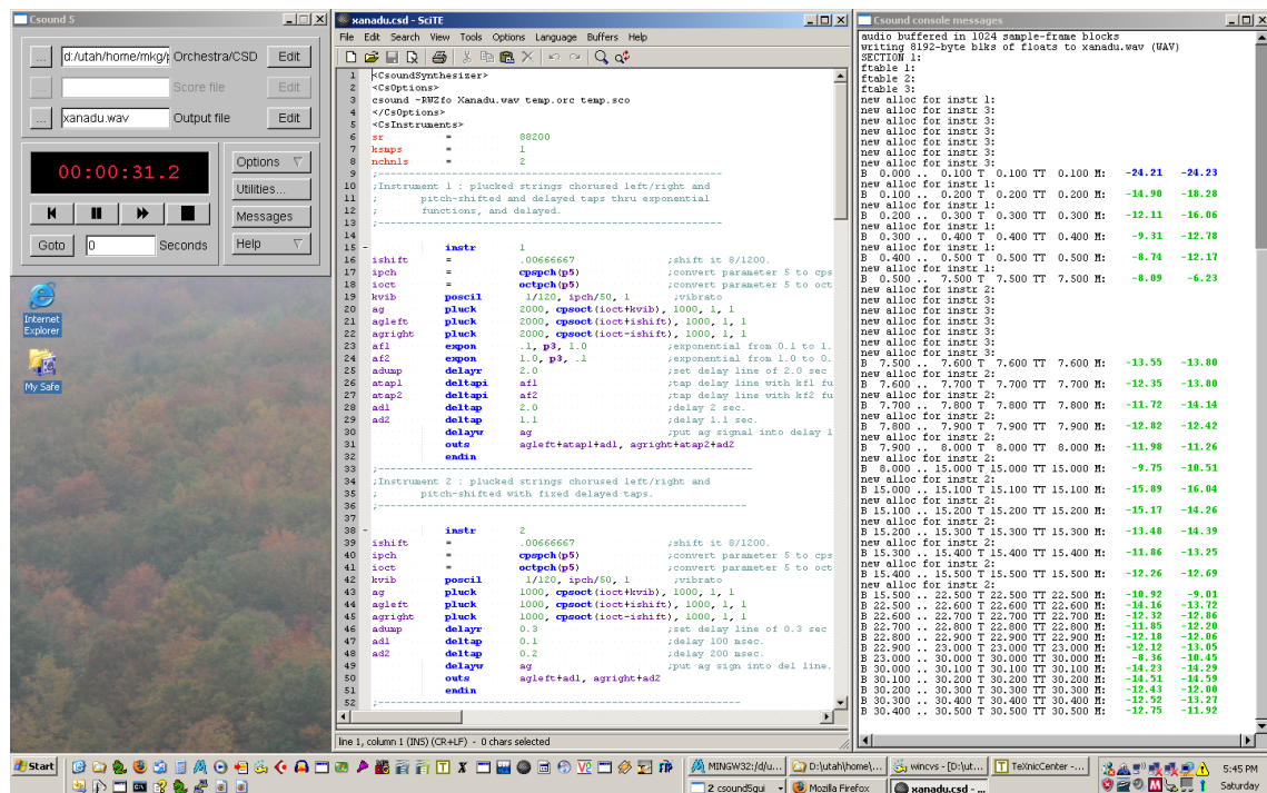
Figure 2.14.: GUI Rendering
