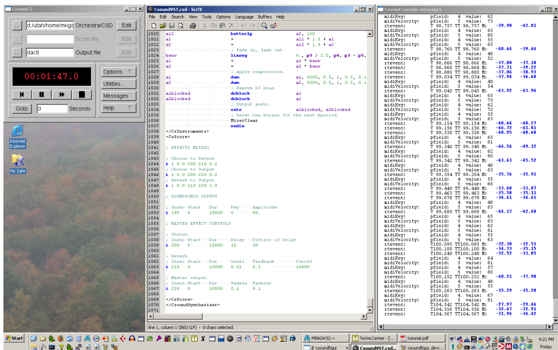
Figure 2.17.: MIDI Performance
