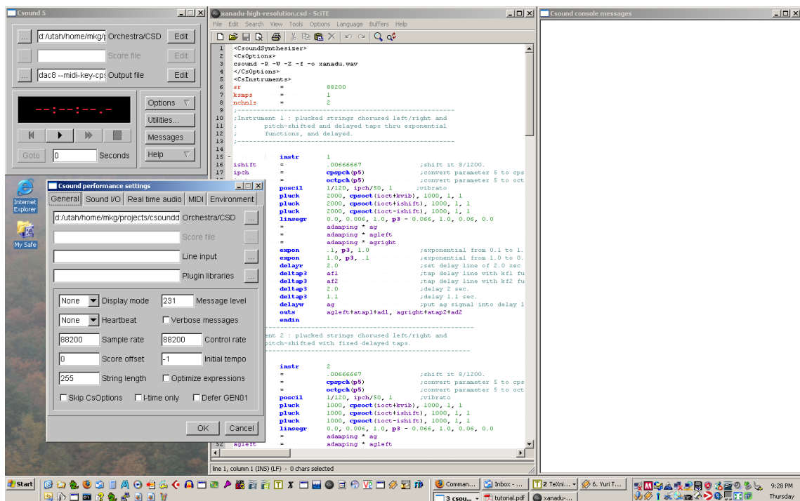
Figure 2.13.: General Options
