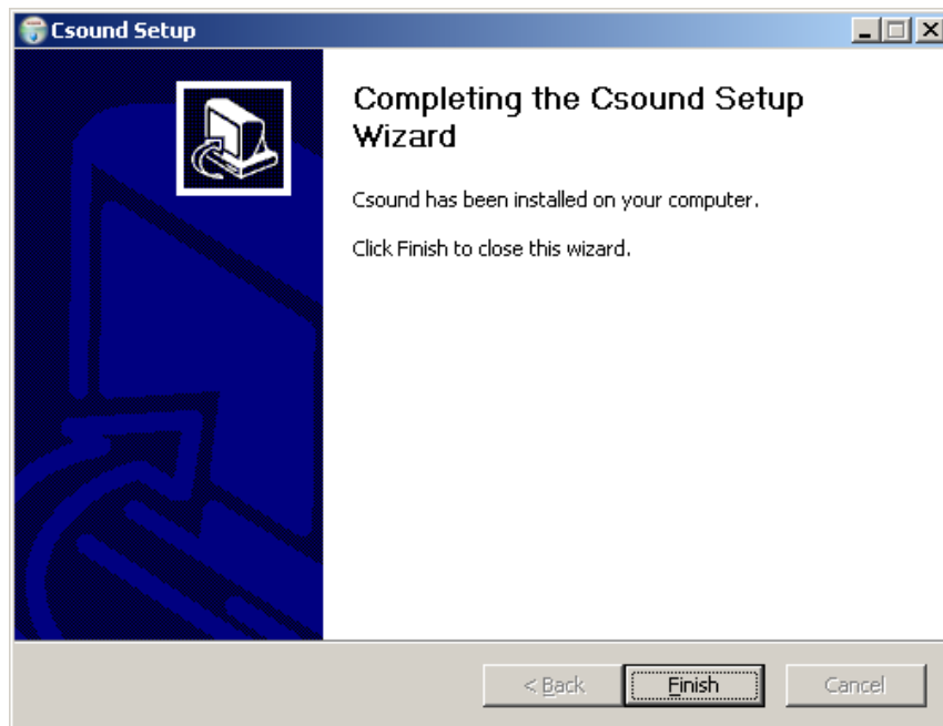
Figure 2.7.: Installation Completed
